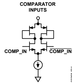
Figure 21. Comparator Inputs
