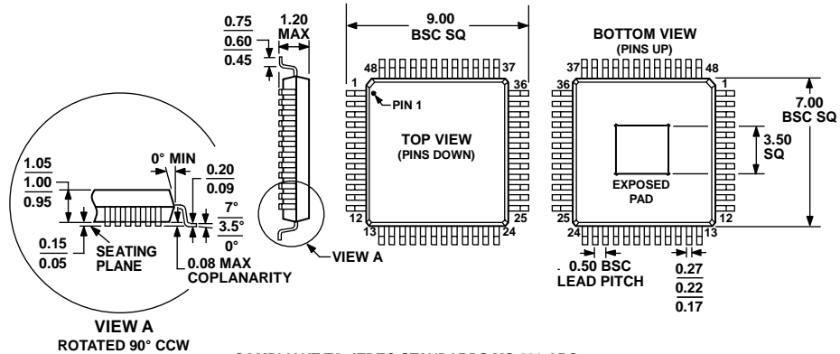
COMPLIANT TO JEDEC STANDARDS MS-026-ABC Figure 33. 48-Lead Thin Quad Flat Package, Exposed Pad [TQFP_EP] (SV-48-4) Dimensions shown in millimeters
