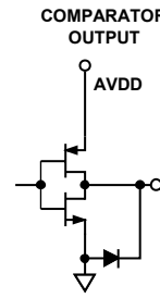
Figure 22. Comparator Outputs
