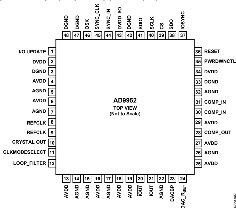
Figure 2. Pin Configuration
